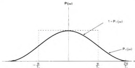
Figure 8.31 Odd symmetry around \omega = \pi/T , as defined in eq. (8.29).
