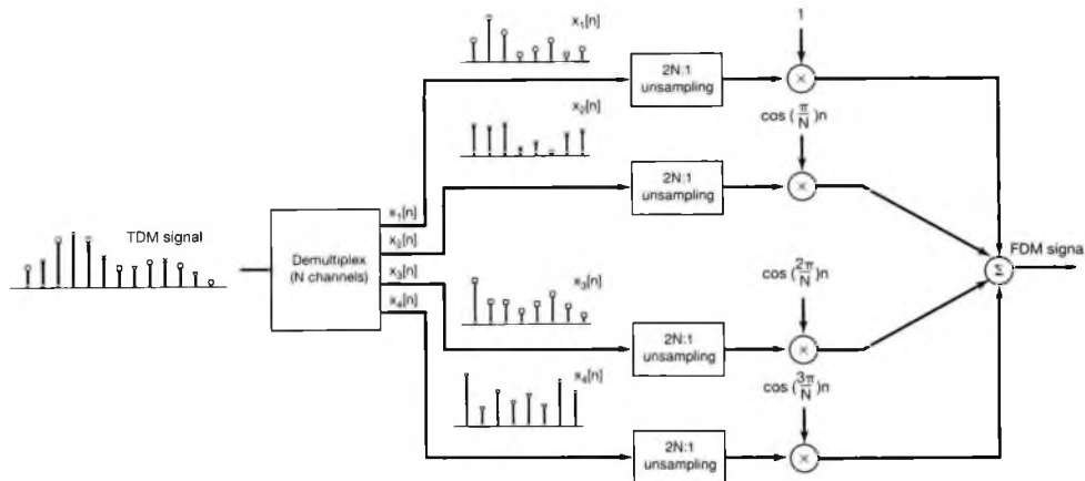
Figure 8.44 Block diagram for TDM-to-FDM transmultiplexing.
