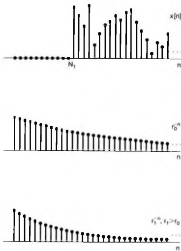
Figure 10.7 With r_1 > r_0 , x[n] decays faster with increasing n than does x[n]r_0^{-n} . Since x[n]r_0^{-n} is absolutely summable, then x[n]r_1^{-n} will also be.
