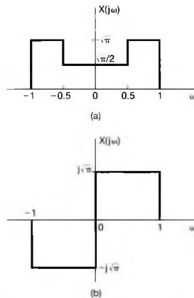
Figure 4.18 The Fourier transforms considered in Example 4.14.
