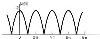
Figure 1.22 The full-wave rectified sinusoid of Example 1.5.
