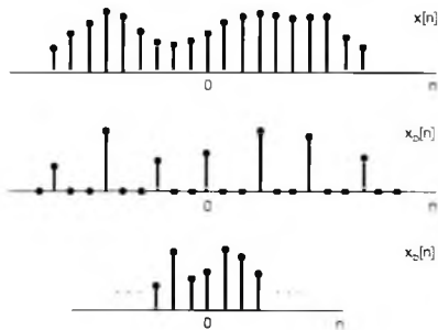
Figure 7.34 Relationship between x_c[n] corresponding to sampling and x_b[n] corresponding to decimation.
