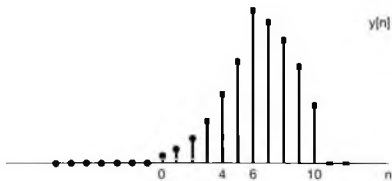
Figure 2.10 Result of performing the convolution in Example 2.4.
