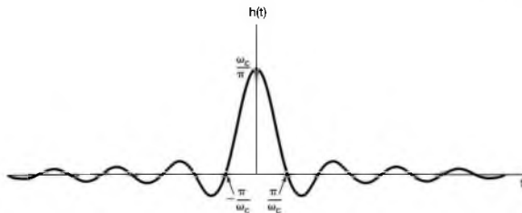
Figure 4.21 Impulse response of an ideal lowpass filter.
