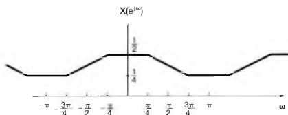
Figure 5.20 Result of the periodic convolution in Example 5.15.
