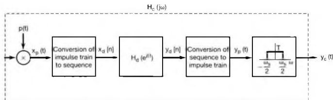
Figure 7.24 Overall system for filtering a continuous-time signal using a discrete-time filter.
