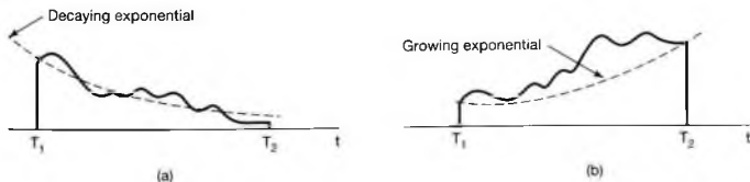
Figure 9.5 (a) Finite-duration signal of Figure 9.4 multiplied by a decaying exponential; (b) finite-duration signal of Figure 9.4 multiplied by a growing exponential.
