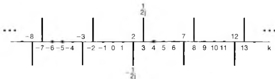
Figure 3.14 Fourier coefficients for x[n] = \sin 3(2\pi/5)n .
