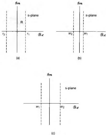
Figure 9.24 Effect on the ROC of time scaling: (a) ROC of X(s) ; (b) ROC of (1/|a|)X(s/a) for 0 < a < 1 ; (c) ROC of (1/|a|)X(s/a) for 0 > a > -1 .
