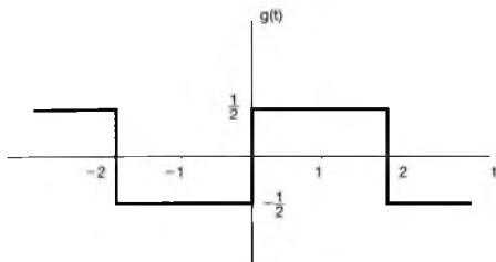
Figure 3.10 Periodic signal for Example 3.6.
