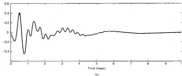
Figure 6.7 Impulse responses associated with the group delay and magnitude characteristics in Figure 6.6: (a) impulse response corresponding to the short-distance category of toll calls; (b) impulse response for the medium-distance category.
