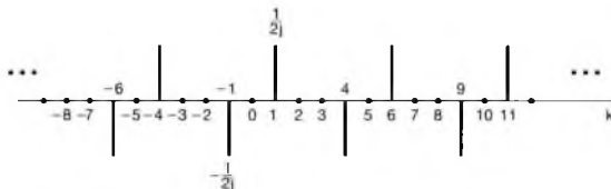
Figure 3.13 Fourier coefficients for x[n] = \sin(2\pi/5)n .
