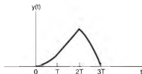
Figure 2.21 Signal y(t) = x(t) * h(t) for Example 2.7.
