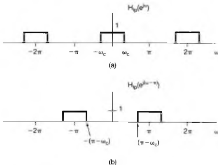
Figure 5.12 (a) Frequency response of a lowpass filter; (b) frequency response of a highpass filter obtained by shifting the frequency response in (a) by \omega = \pi corresponding to one-half period.
