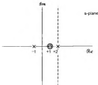
Figure 9.3 Pole-zero plot and ROC for Example 9.5.
