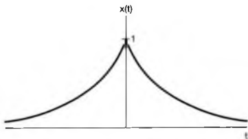
Figure 4.6 Signal x(t) = e^{-a|t|} of Example 4.2.
