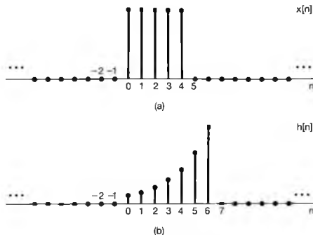
Figure 2.8 The signals to be convolved in Example 2.4.
