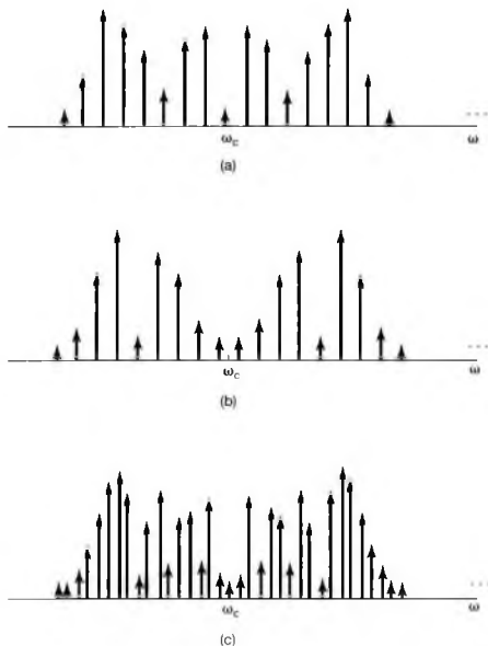
Figure 8.35 Magnitude of spectrum of wideband frequency modulation with m = 12 : (a) magnitude of spectrum of \cos \omega_c t \cos[m \sin \omega_m t] ; (b) magnitude of spectrum of \sin \omega_c t \sin[m \sin \omega_m t] ; (c) combined spectral magnitude of y(t) .
