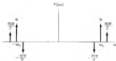
Figure 8.33 Approximate spectrum for narrowband FM.
