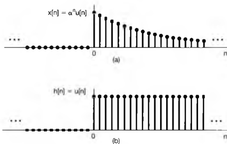
Figure 2.5 The signals x[n] and h[n] in Example 2.3.
