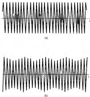
Figure 8.34 Comparison of narrowband FM and AM-DSB/SC: (a) narrowband FM; (b) AM-DSB/SC.
