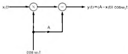
Figure 8.12 Modulator for an asynchronous modulation-demodulation system.
