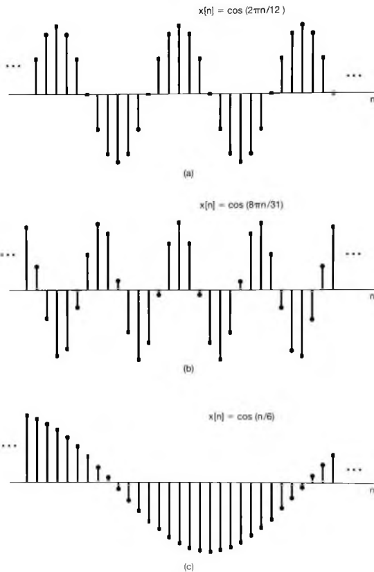
Figure 1.25 Discrete-time sinusoidal signals.
