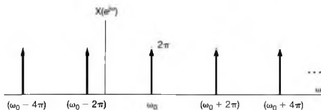
Figure 5.8 Fourier transform of x[n] = e^{j\omega_0 n} .
