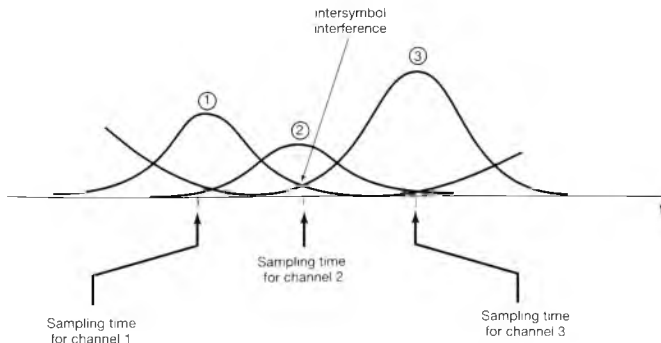
Figure 8.28 Intersymbol interference.
