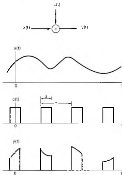
Figure 8.23 Amplitude modulation of a pulse train.
