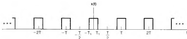
Figure 4.1 A continuous-time periodic square wave.
