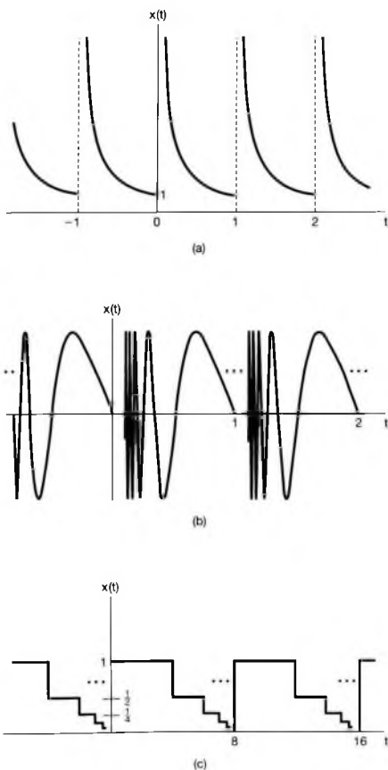
Figure 3.8 Signals that violate the Dirichlet conditions: (a) the signal x(t) = 1/t for 0 < t \leq 1 , a periodic signal with period 1 (this signal violates the first Dirichlet condition); (b) the periodic signal of eq. (3.57), which violates the second Dirichlet condition; (c) a signal periodic with period 8 that violates the third Dirichlet condition [for 0 \leq t < 8 , the value of x(t) decreases by a factor of 2 whenever the distance from t to 8 decreases by a factor of 2; that is, x(t) = 1 , 0 \leq t < 4 , x(t) = 1/2 , 4 \leq t < 6 , x(t) = 1/4 , 6 \leq t < 7 , x(t) = 1/8 , 7 \leq t < 7.5 , etc.].
