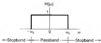
Figure 4.20 Frequency response of an ideal lowpass filter.
