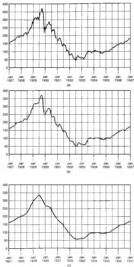
Figure 6.36 Effect of lowpass filtering on the Dow Jones weekly stock market index over a 10-year period using moving-average filters: (a) weekly index; (b) 51-day moving average applied to (a); (c) 201-day moving average applied to (a). The weekly stock market index and the two moving averages are discrete-time sequences. For clarity in the graphical display, the three sequences are shown here with their individual values connected by straight lines to form a continuous curve.
