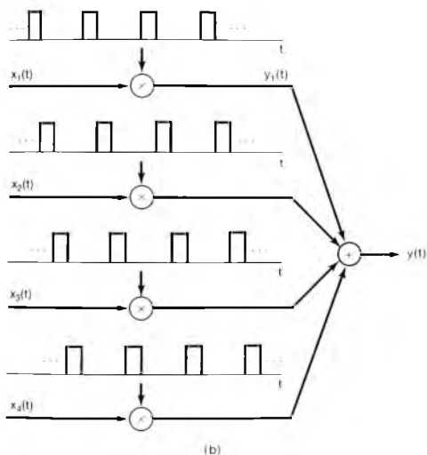
Figure 8.25 Time-division multiplexing.
