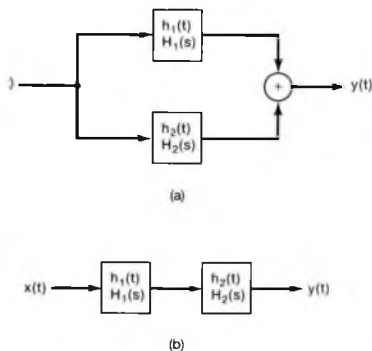
Figure 9.30 (a) Parallel interconnection of two LTI systems; (b) series combination of two LTI systems.
