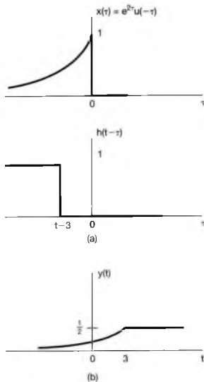
Figure 2.22 The convolution problem considered in Example 2.8.
