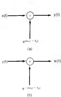
Figure 8.7 System for amplitude modulation and demodulation using a complex exponential carrier: (a) modulation; (b) demodulation.
