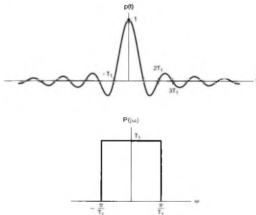
Figure 8.29 A sinc pulse and its corresponding spectrum
