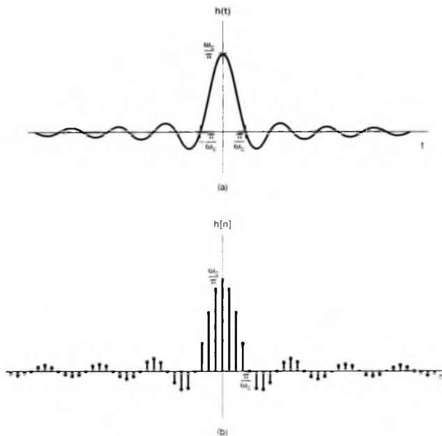
Figure 6.12 (a) The impulse response of the continuous-time ideal lowpass filter of Figure 6.10(a); (b) the impulse response of the discrete-time ideal lowpass filter of Figure 6.10(b) with \omega_c = \pi/4 .
