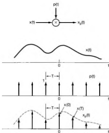
Figure 7.2 Impulse-train sampling.
