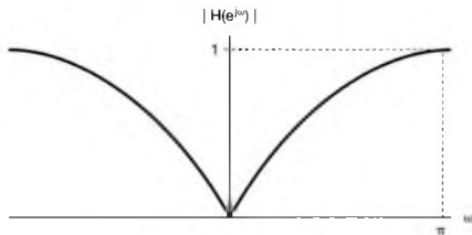
Figure 3.37 Frequency response of a simple highpass filter.
