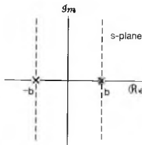
Figure 9.12 Pole-zero plot and ROC for Example 9.7.
