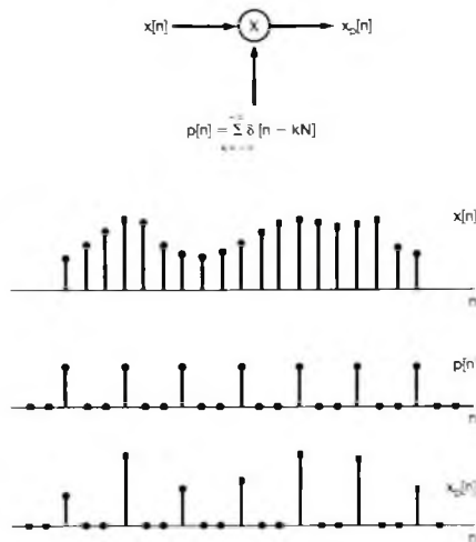
Figure 7.31 Discrete-time sampling.
