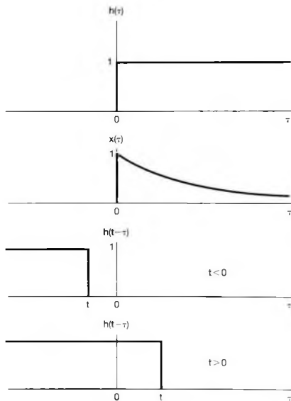
Figure 2.17 Calculation of the convolution integral for Example 2.6.
