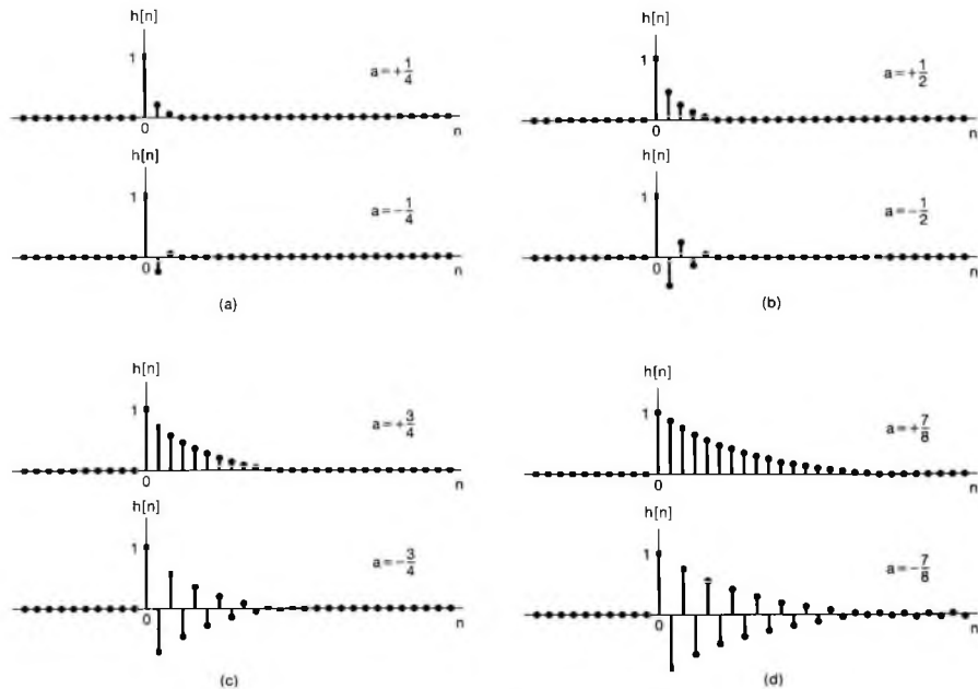
Figure 6.26 Impulse response h[n] = a^n u[n] of a first-order system: (a) a = \pm 1/4 ; (b) a = \pm 1/2 ; (c) a = \pm 3/4 ; (d) a = \pm 7/8 .
