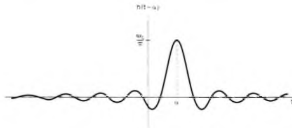
Figure 6.13 Impulse response of an ideal lowpass filter with magnitude and phase shown in Figure 6.11.
