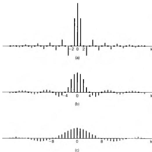
Figure 3.7 Plots of the scaled Fourier series coefficients T_n for the periodic square wave with T_1 fixed and for several values of T : (a) T = 4T_1 ; (b) T = 8T_1 ; (c) T = 16T_1 . The coefficients are regularly spaced samples of the envelope (2 \sin \omega T_1)/\omega , where the spacing between samples, 2\pi/T , decreases as T increases.
