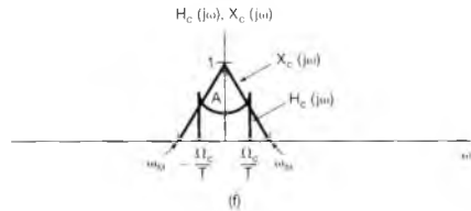
Figure 7.25 Frequency-domain illustration of the system of Figure 7.24: (a) continuous-time spectrum X_c(j\omega) ; (b) spectrum after impulse-train sampling; (c) spectrum of discrete-time sequence x_d[n] ; (d) H_d(e^{j\Omega}) and X_d(e^{j\Omega}) that are multiplied to form Y_d(e^{j\Omega}) ; (e) spectra that are multiplied to form Y_p(j\omega) ; (f) spectra that are multiplied to form Y_c(j\omega) .
