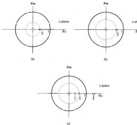
Figure 10.4 Pole-zero plot and region of convergence for the individual terms and the sum in Example 10.3: (a) 1/(1 - \frac{1}{3}z^{-1}) , |z| > \frac{1}{3} ; (b) 1/(1 - \frac{1}{2}z^{-1}) , |z| > \frac{1}{2} ; (c) 7/(1 - \frac{1}{3}z^{-1}) - 6/(1 - \frac{1}{2}z^{-1}) , |z| > \frac{1}{2} .
