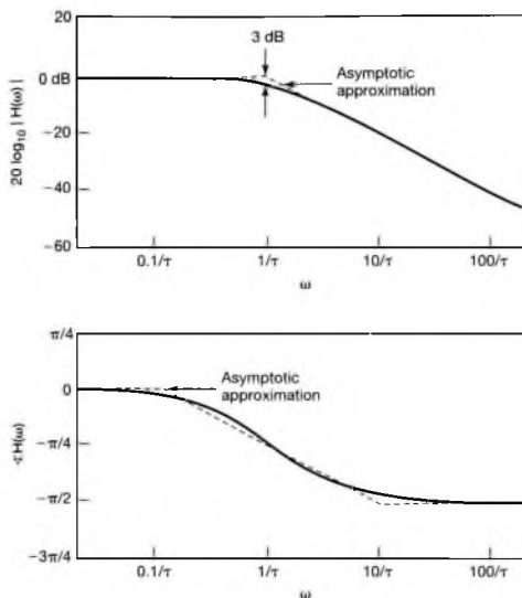
Figure 9.18 Frequency response for a first-order system.
