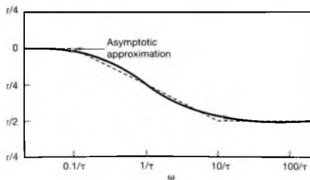
Figure 6.20 Bode plot for a continuous-time first-order system.
