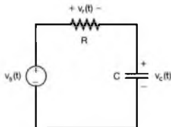
Figure 3.29 First-order RC filter.
