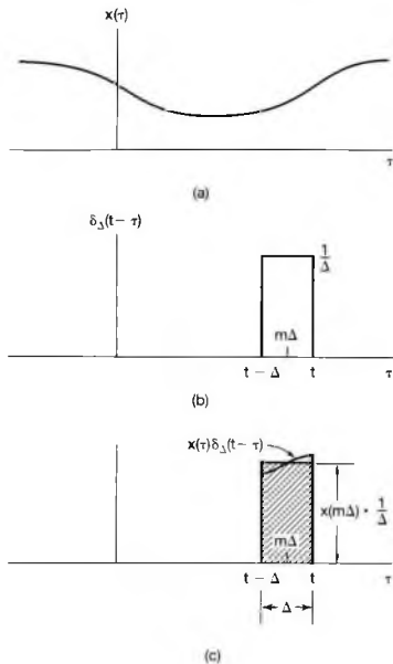
Figure 2.13 Graphical interpretation of eq. (2.26).
