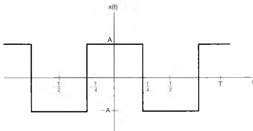
Figure 8.36 Symmetric periodic square wave.
