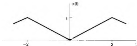
Figure 3.11 Triangular wave signal in Example 3.7.
