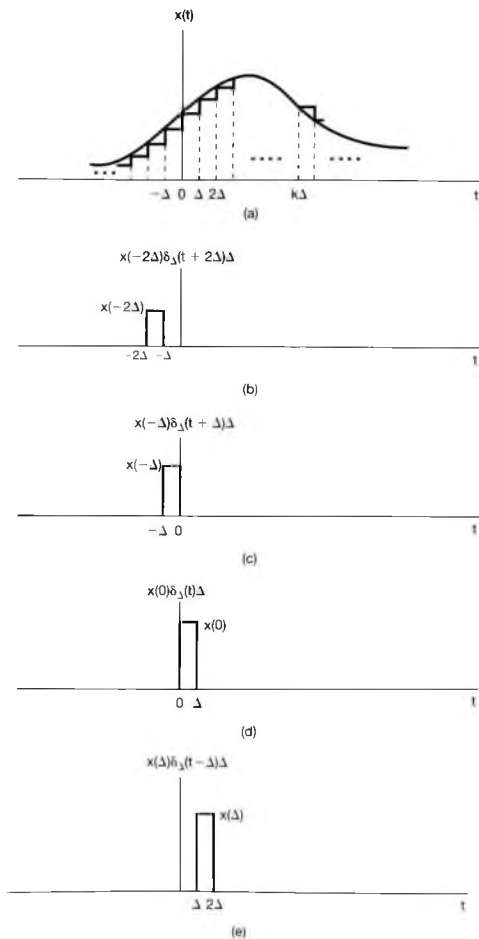
Figure 2.12 Staircase approximation to a continuous-time signal.
