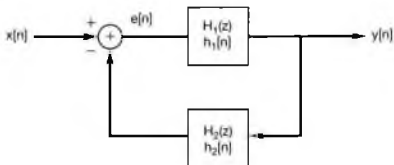
Figure 10.17 Feedback interconnection of two systems.
