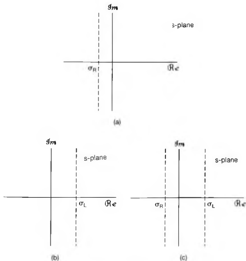
Figure 9.10 (a) ROC for x_R(t) in Figure 9.9; (b) ROC for x_L(t) in Figure 9.9; (c) the ROC for x(t) = x_R(t) + x_L(t) , assuming that the ROCs in (a) and (b) do not overlap.
