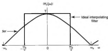
Figure 7.11 Transfer function for the zero-order hold and for the ideal interpolating filter.
