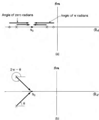
Figure 11.13 (a) Angle contribution from real poles and zeros to a point on the real axis. (b) total angle contribution from a complex-conjugate pole-zero pair to a point on the real axis.
