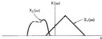
Figure 6.15 Two spectra that are slightly overlapping.
