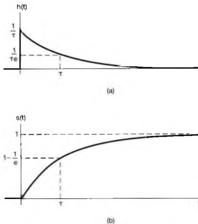
Figure 3.31 (a) Impulse response of the first-order RC lowpass filter with \tau = RC ; (b) step response of RC lowpass filter with \tau = RC .
